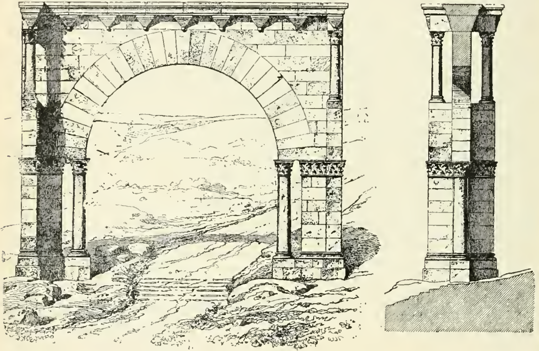
FIG. 56. Deir Siman, Syria: Triumphal arch built in the sixth century.
