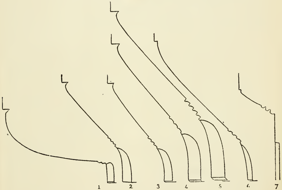
FIG. 12. Profiles of Doric capitals, as follows: Nos. 1 and 6, early capitals found on Acropolis at Athens. No. 2, Athens: so-called Temple of Theseus. No. 3, Athens: Propylaia. Nos. 4 and 5, Athens: Parthenon. No. 7, Cori (Southern Italy): so-called Temple of Hercules.
