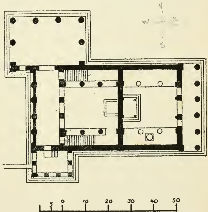
FIG. 14. Athens: Erechtheion. Finished about 407 B.C. Plan.
