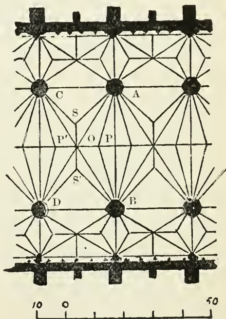
FIG. 134. Lincoln, England: Cathedral. Plan of nave vaulting. About 1235 A.D.
