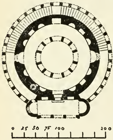
FIG. 61. Rome: Church of S. Constanza; originally a tomb-chapel. About 315 A.D.
