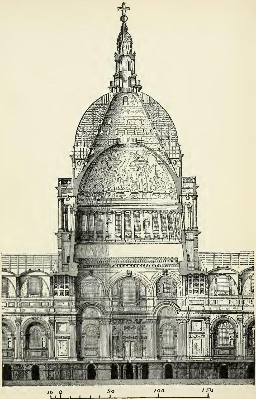
FIG. 251. London: S. Paul's. 1680 to 1710. Part of longitudinal section.
