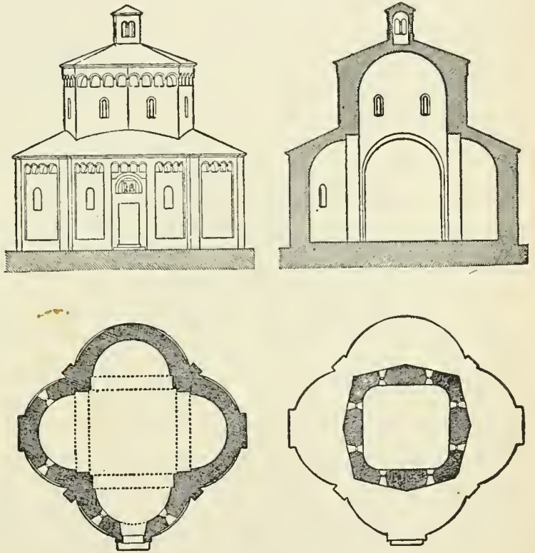
FIG. 65. Biella, Italy: Chapel probably of the eighth century A.D.
