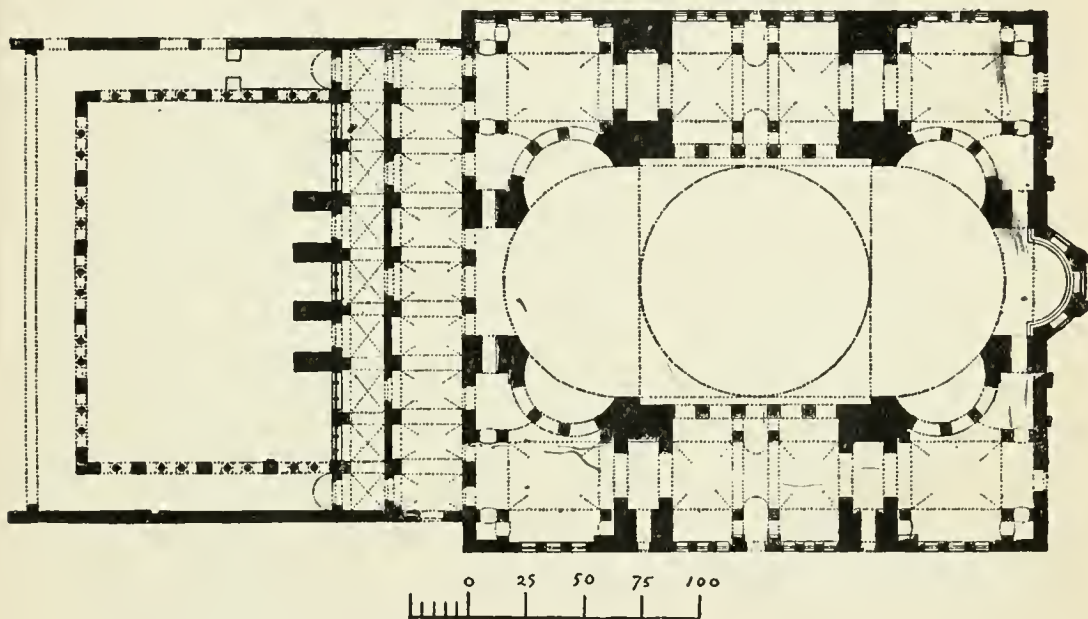
FIG. 68. Constantinople: Church of Hagia Sophia, rebuilt 561.
