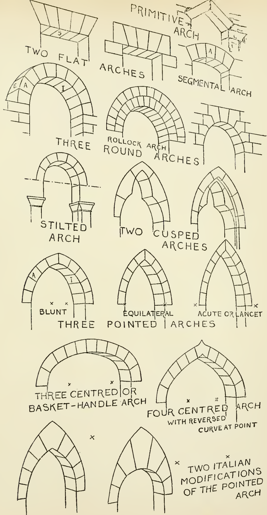
PLATE X. Illustrations of term "Arch" in Glossary.
