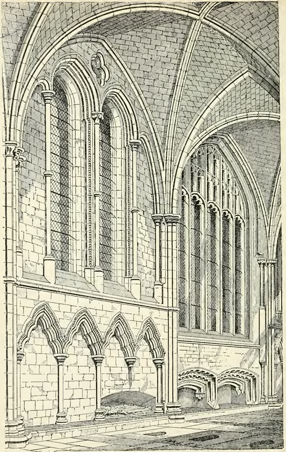
FIG. 136. Carlisle, England: Cathedral. Two bays of north aisle of choir.
