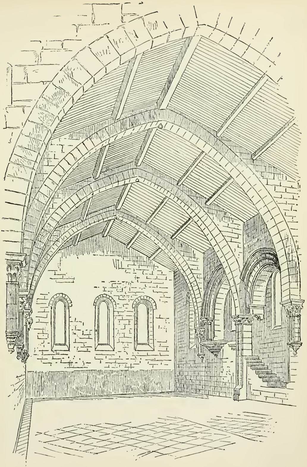
FIG. 138 A. Fossanova, Italy: Refectory. About 1205 A.D.
