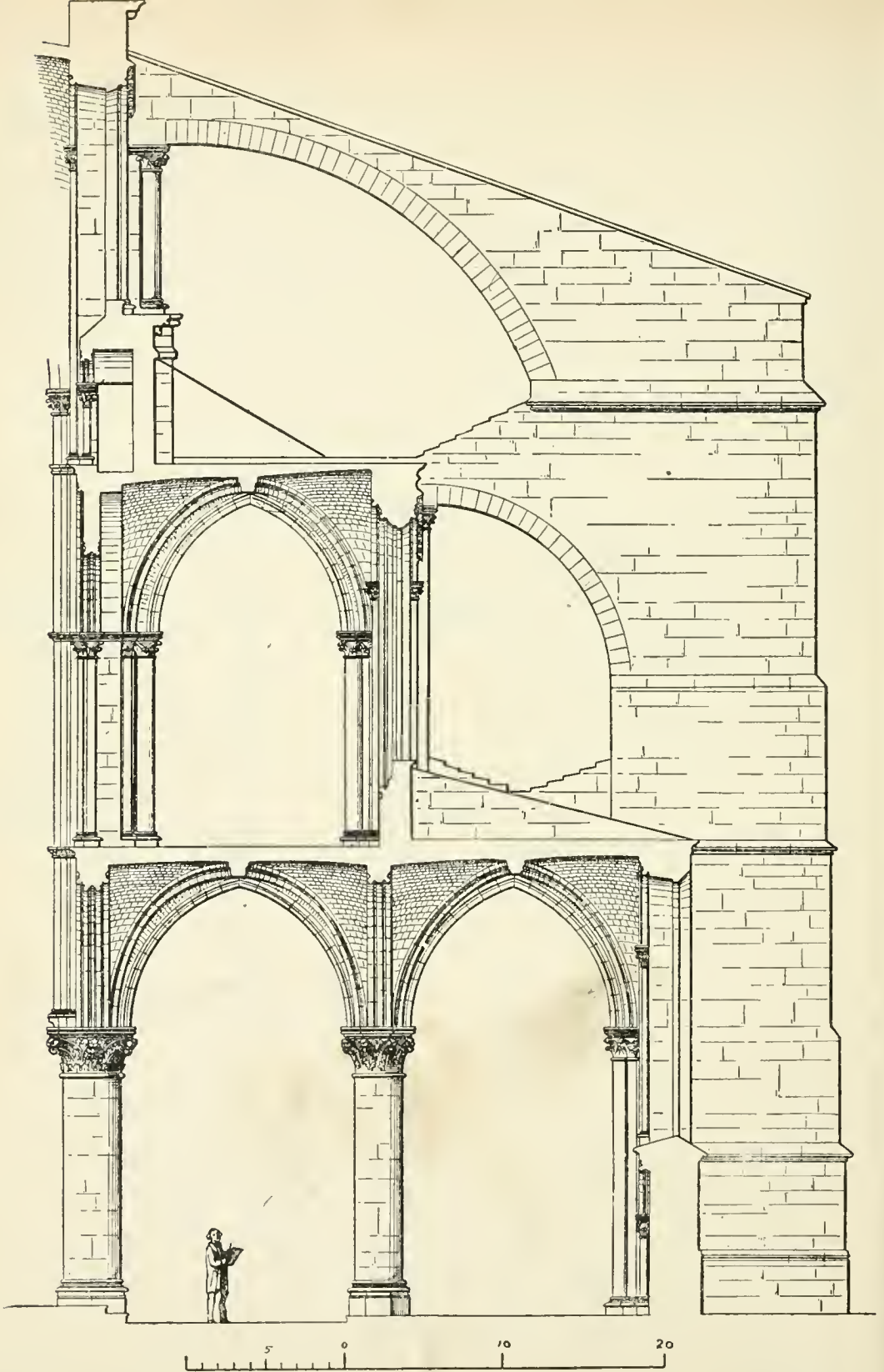
FIG. 117. Reims, France: S. Remy. Section across choir with butress-system of twelfth century.
