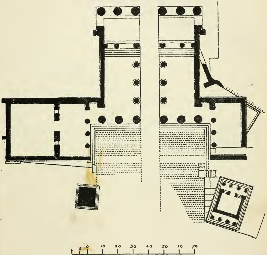
FIG. 7. Athens: Propylaea of Acropolis. 437 to 432 B.C. Plan.
