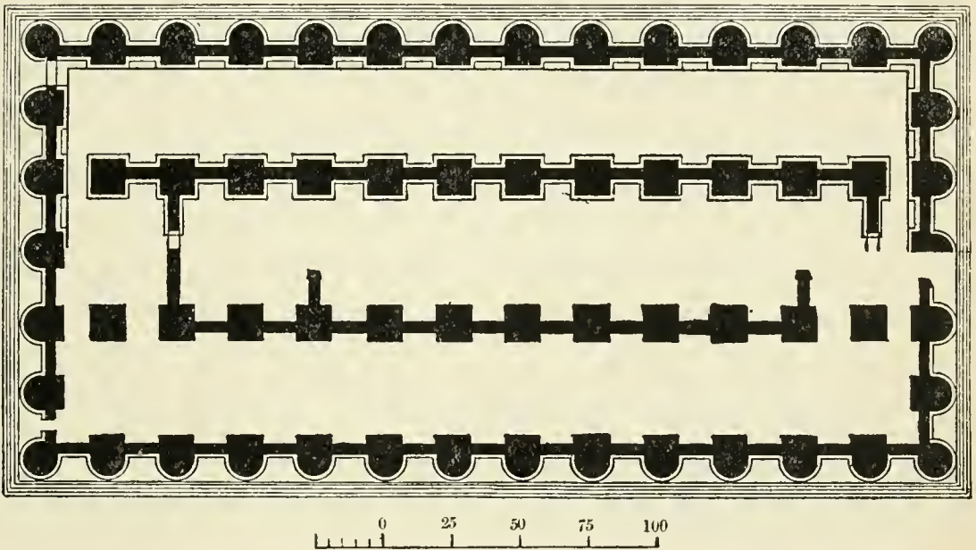
FIG. 27. Girgenti, Sicily: ruins of Akragas. Temple of Zeus. Approximate plan.
